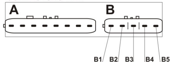
CONNECTORS VIEW
